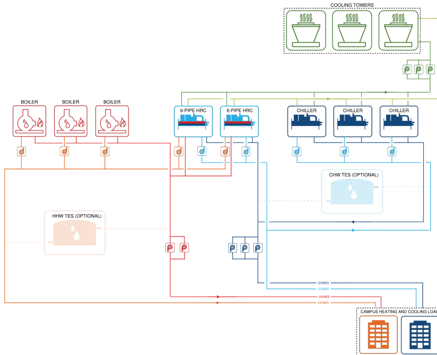
Figure 5.9: Centralized Heat Recovery Strategy Schematic
