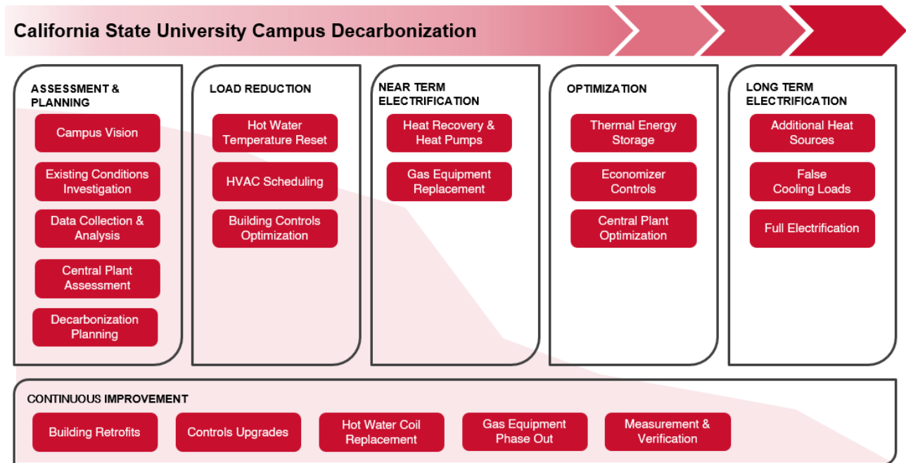
Figure 5.1: CSU System Decarbonization Framework
