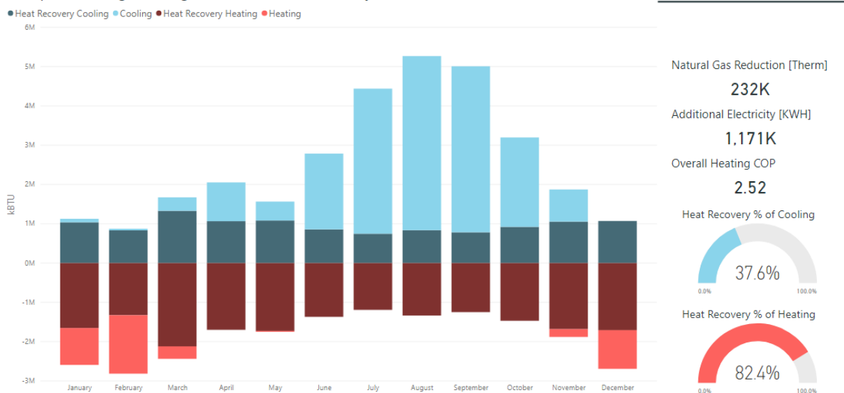
Campus Cooling Heating Profile w/ Heat Recovery Chiller & TES
