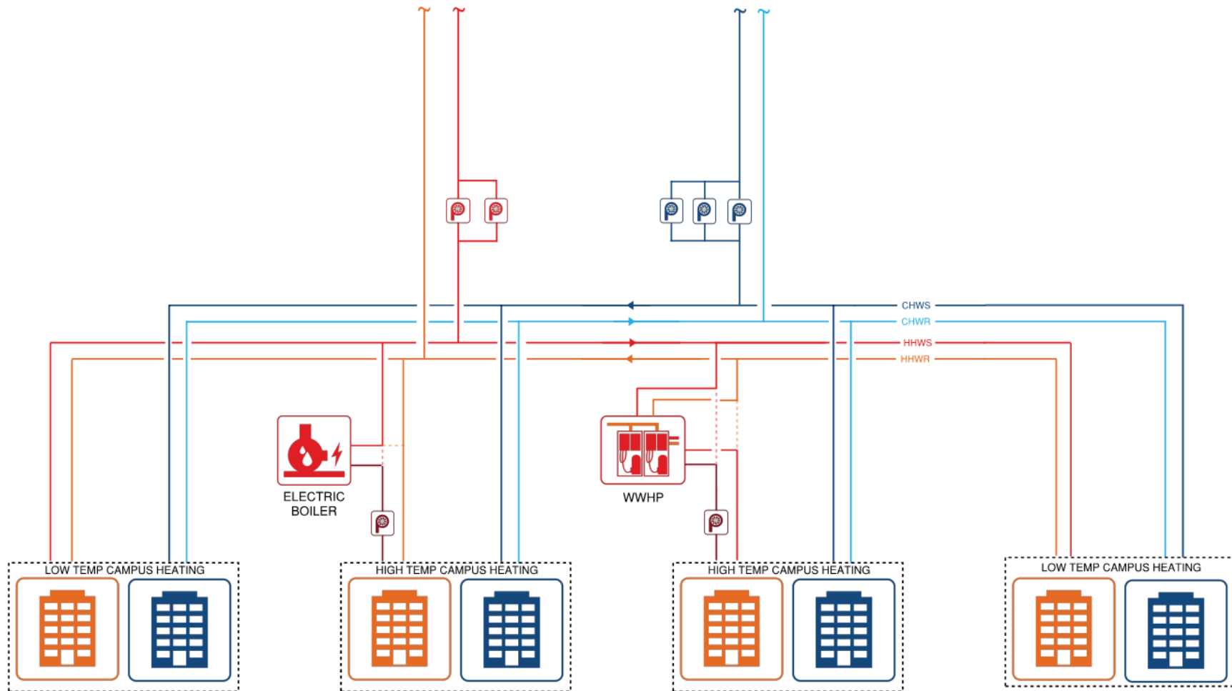
Figure 5.15: Cascade Style Heating Schematic
