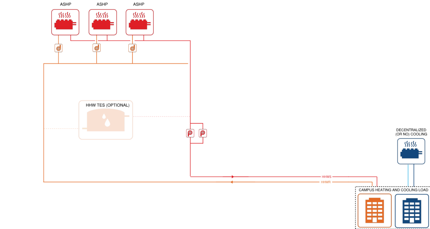
Figure 5.11: Centralized Heat Pump Strategy Schematic
