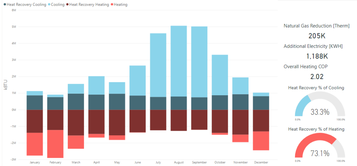
Figure 5.6: Heat Recovery Potential
