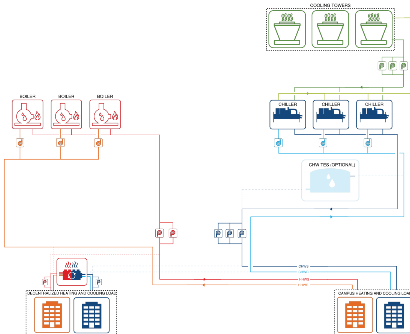
Figure 5.10: Decentralized Heat Recovery Strategy Schematic
